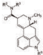
Ergot alkaloids
