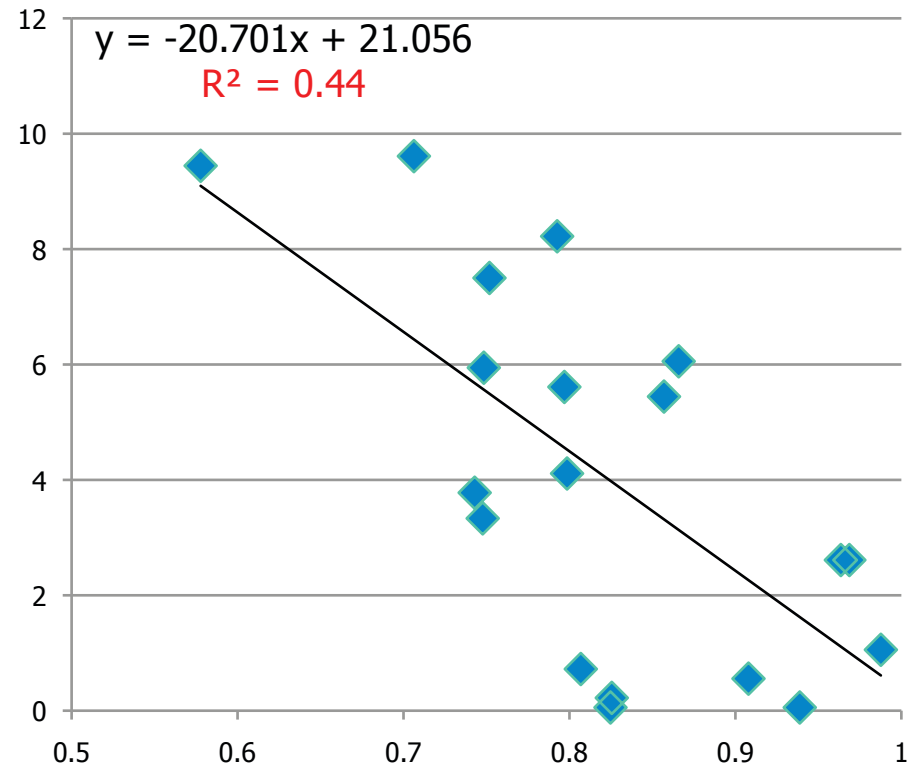
142% Stocking Density
