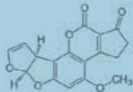
Aflatoxins
