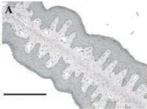
High Grain
