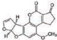
Aflatoxins
