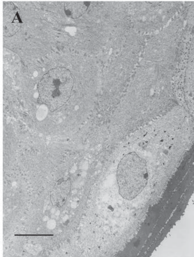
High Forage
