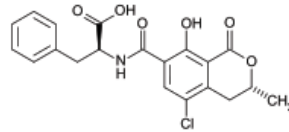
Ochratoxin A
